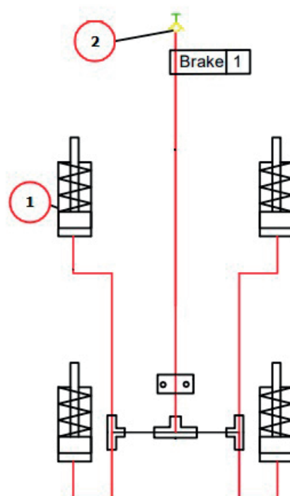
Bromsschema
