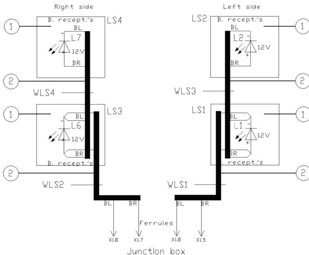
Koblingsdiagram for sidemarkeringslysene
