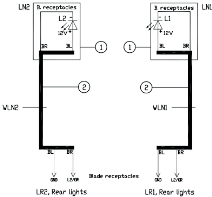
Koblingsdiagram for skiltlysene
