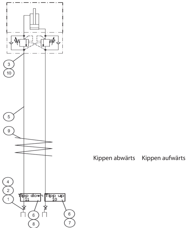
Hydraulikschema BIGAB 7-10 – 14-17
